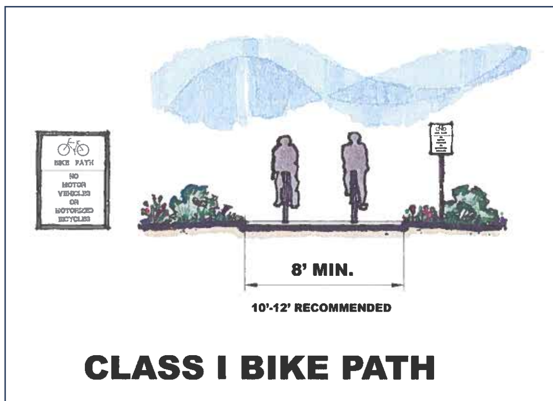
FIGURE E.3 - CLASS I BIKE PATH
